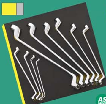
10 ringsleutels, 6x7, 8x9, 10x11, 12x13, 14x15, 16x17, 18x21, 19x22, 24x27 en 30x32 mm
